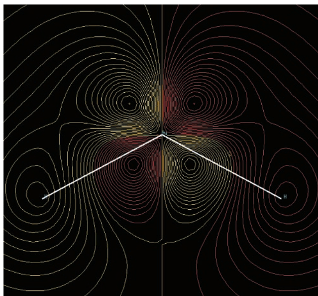
Figure 4. Two-dimensional electron density contour plot of the AuH 2 ground state. Calculation at MP2 level with 3s3p4d2f basis for gold and CCPVTZ basis for hydrogen.
